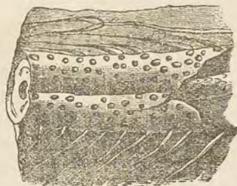
STIGMARIA FICOÏDES, (One fourth nat. size.)
